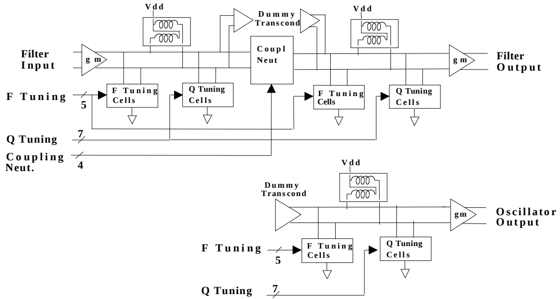
Figure 1. Chip Architecture.
